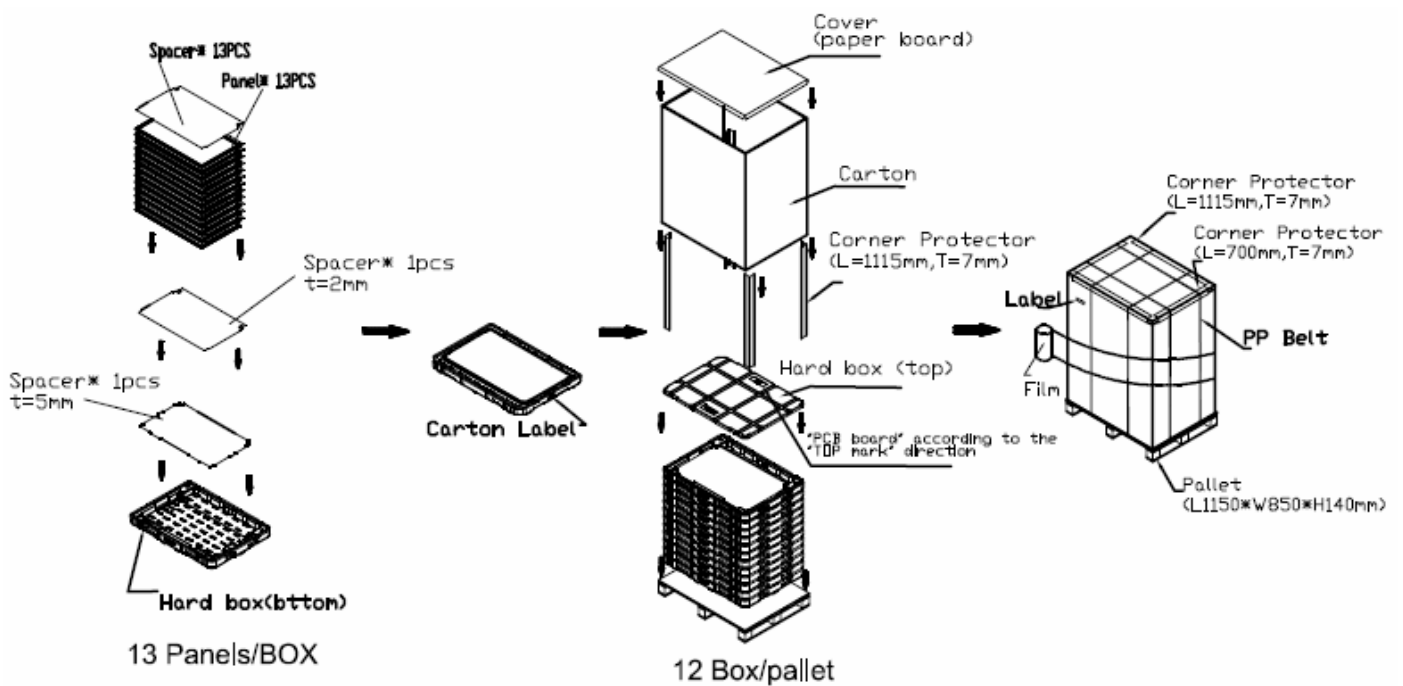
Figure.10-1 packing method
