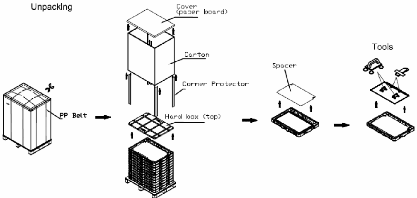
Figure.10-3 unpacking method
