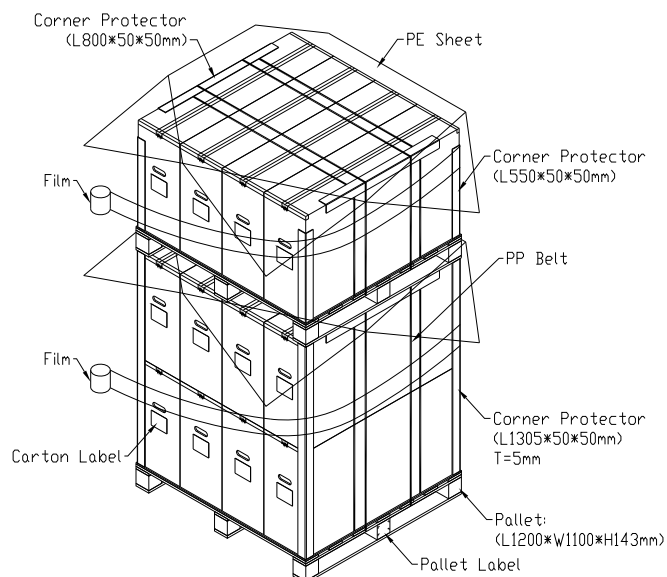
Figure.10-2 packing method
