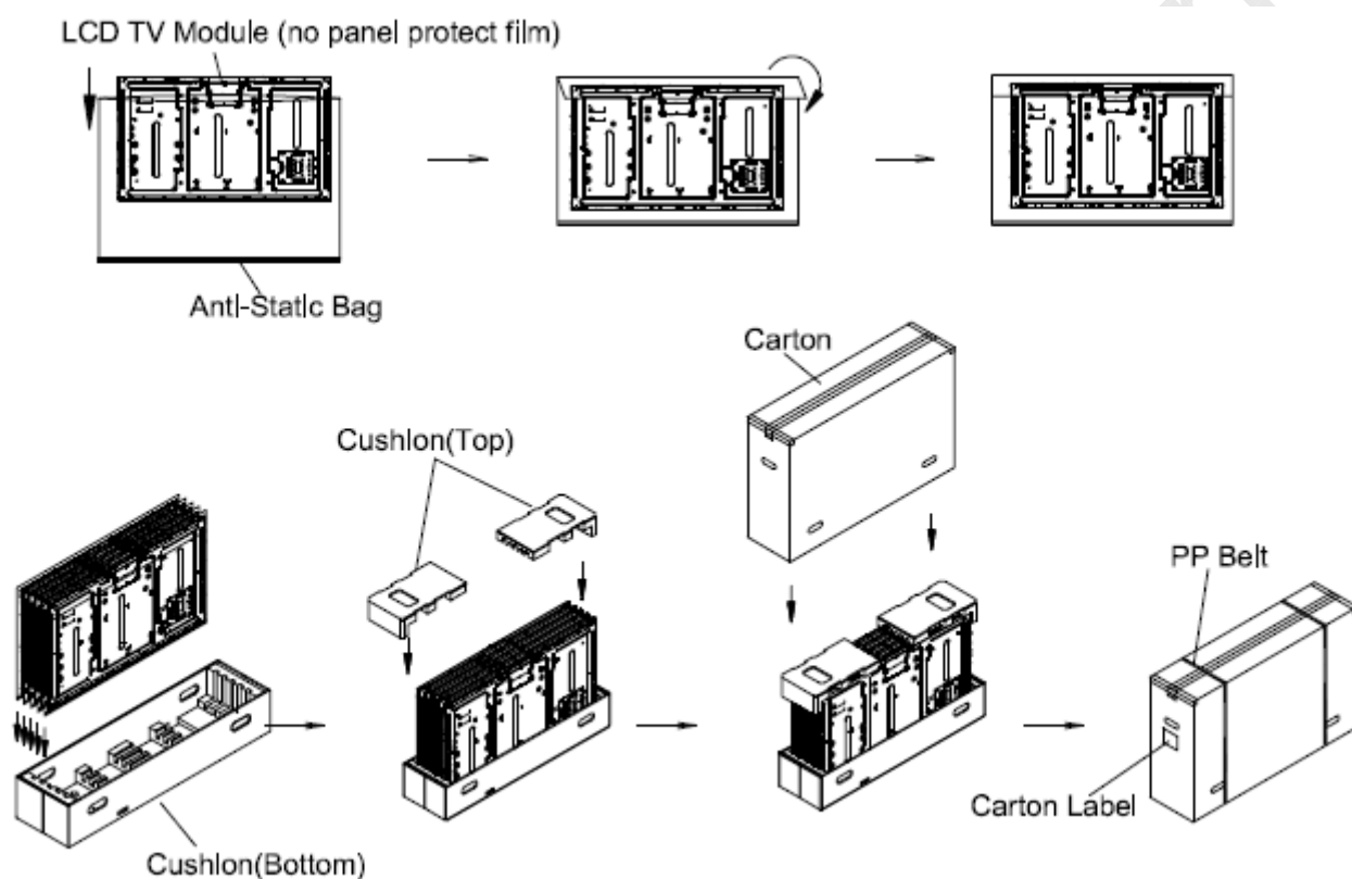
Figure.9-1 packing method
