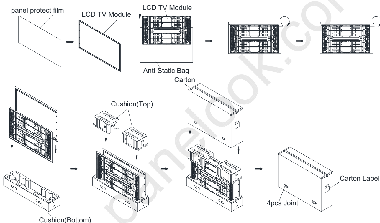
Figure.11-1 packing method
