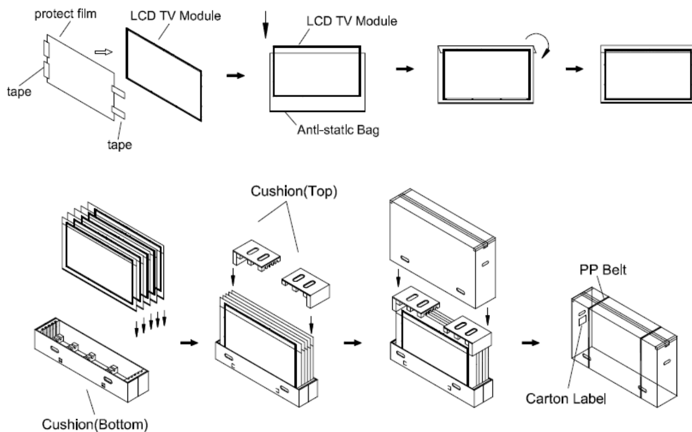
Figure 10-1 packing method
