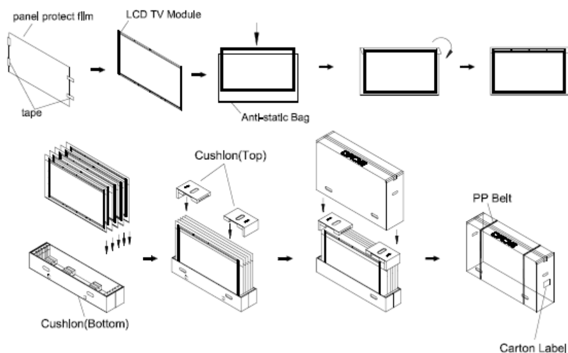
Figure.9-1 packing method
