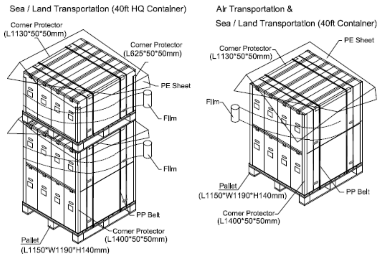
Figure 10-2 packing method
