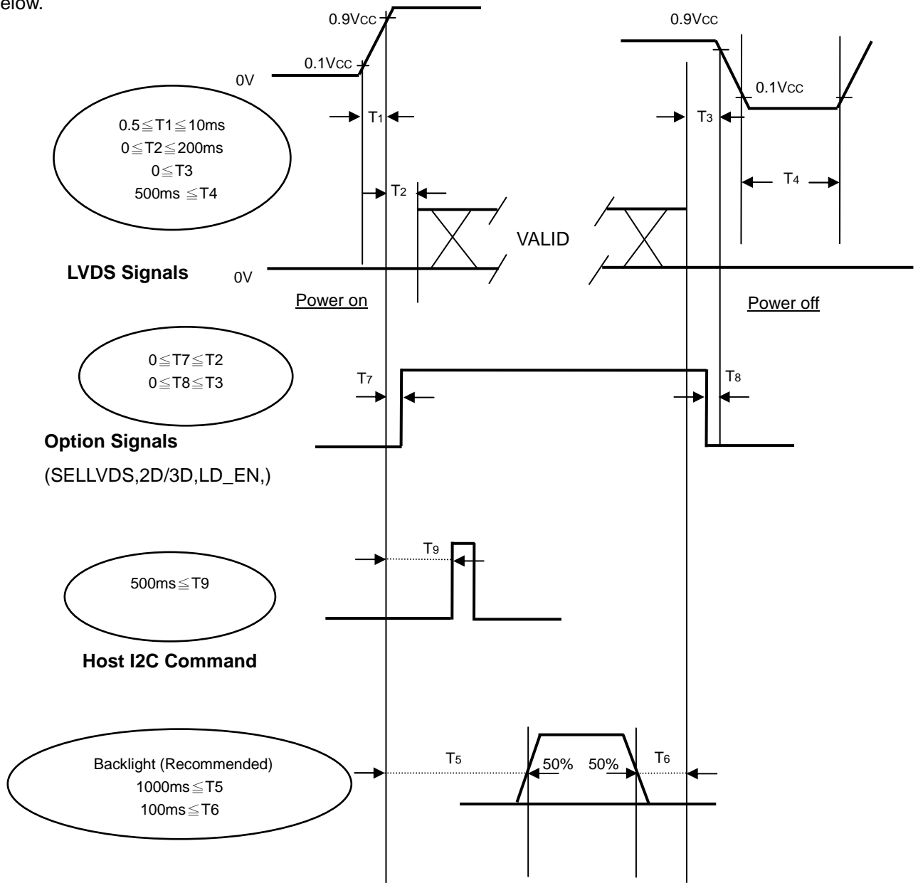
Power ON/OFF Sequence
