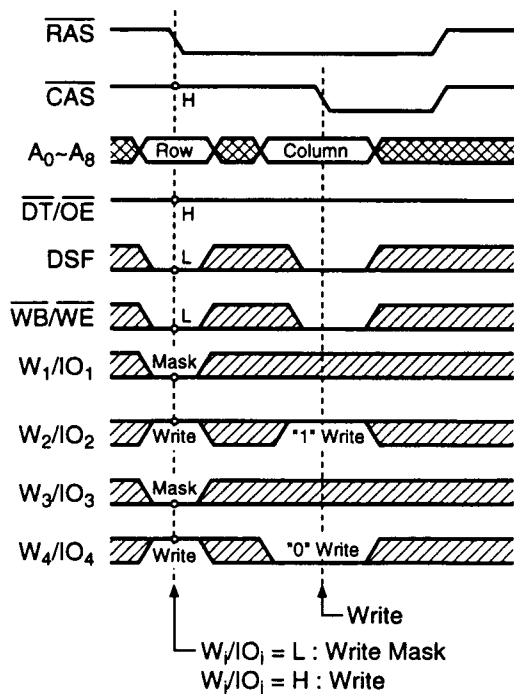
Figure 2. Write-per-bit timing cycle
