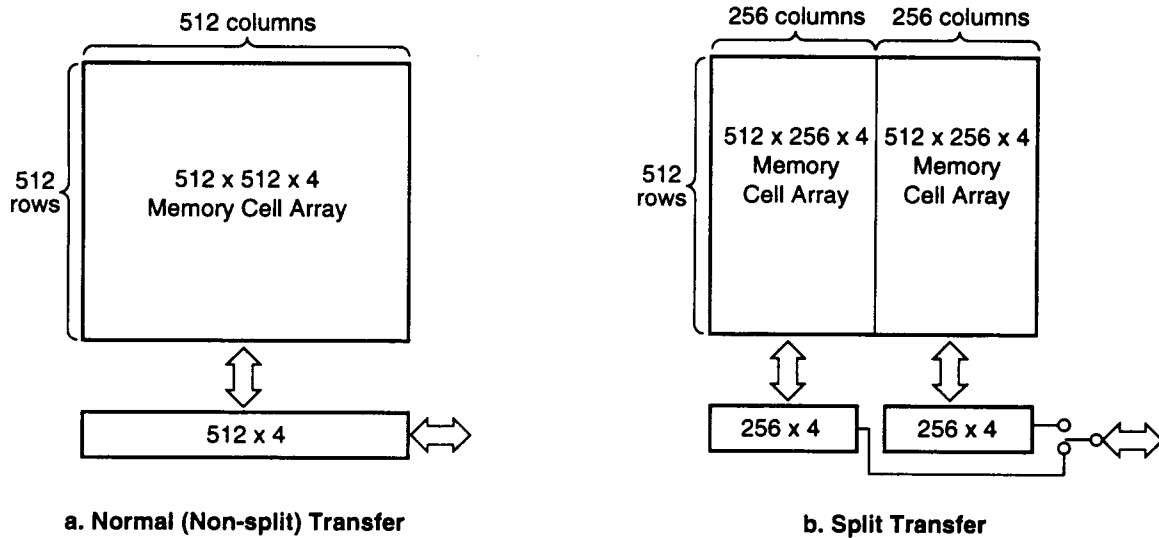
Figure 11. Transfer Operation
