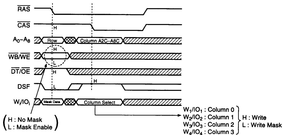
Figure 7. Block Write Timing
