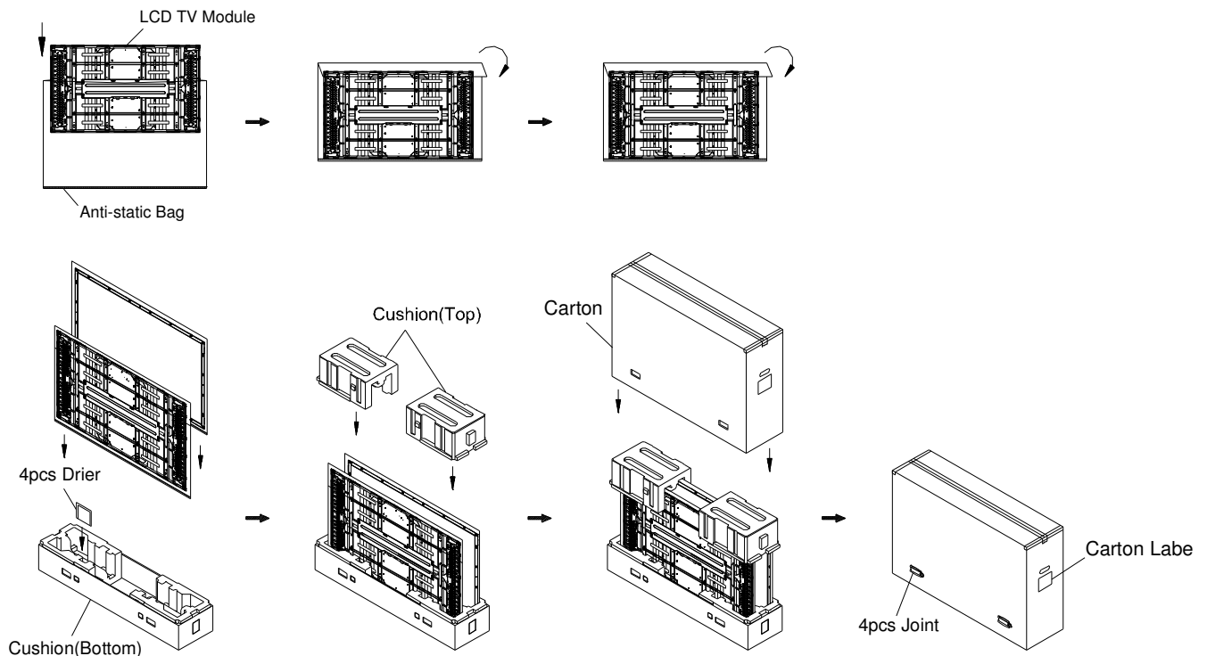
Figure.9-1 packing method
