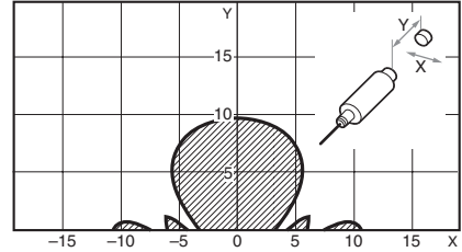
V600-HS51 & V600-D23P55
