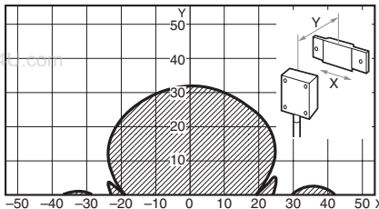
V600-HS63 & V600-D23P66SP
