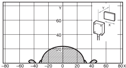
V600-HS63 & V600-D2KR16
