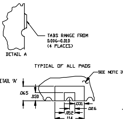
PHYSICAL DIMENSIONS
