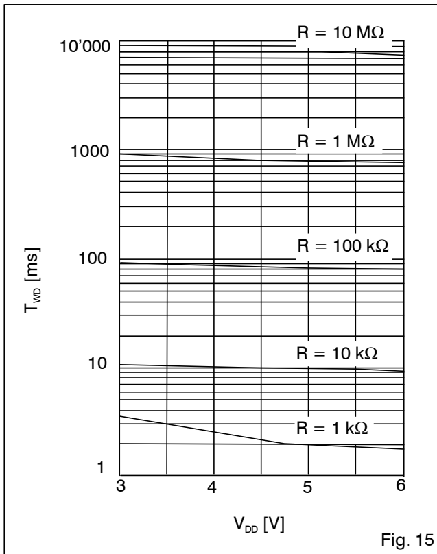
T_{WD} versus V_{DD} at T_A = -40^\circ C
