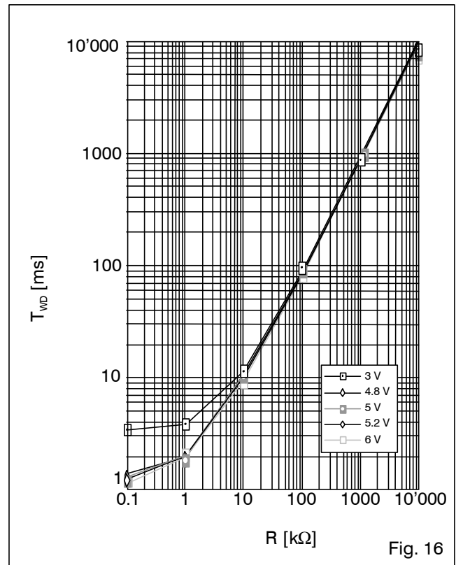
T_{WD} versus R at T_A = -40^\circ C
