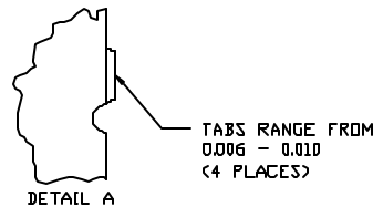
PHYSICAL DIMENSIONS
