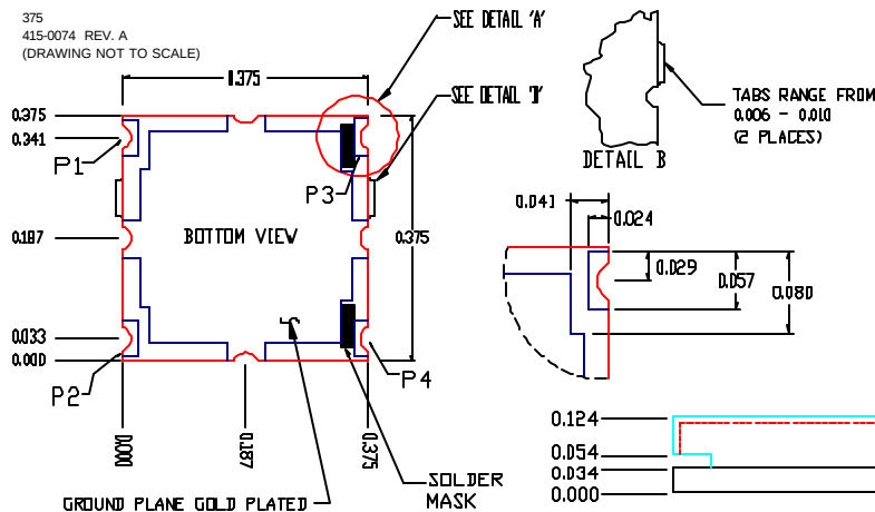
PHYSICAL DIMENSIONS
