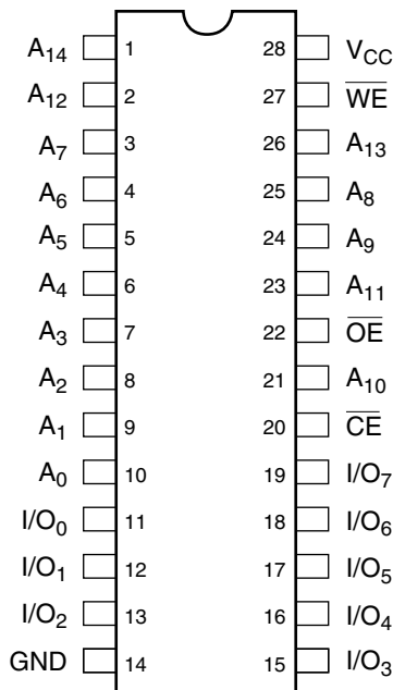
28-Pin SOP
