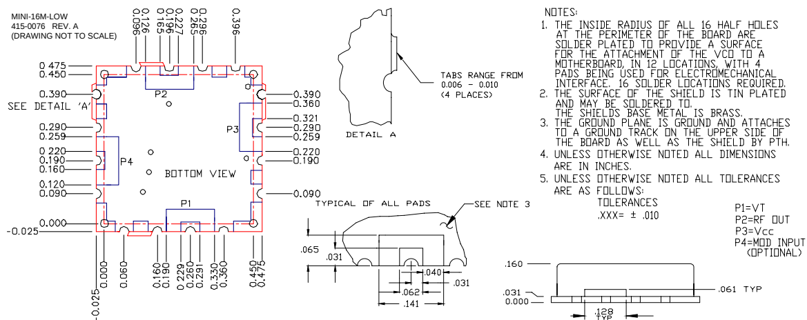
PHYSICAL DIMENSIONS
