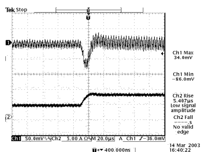
Vout=1.0V 50% to 100% load transients at 5V input and Ta=25° C
