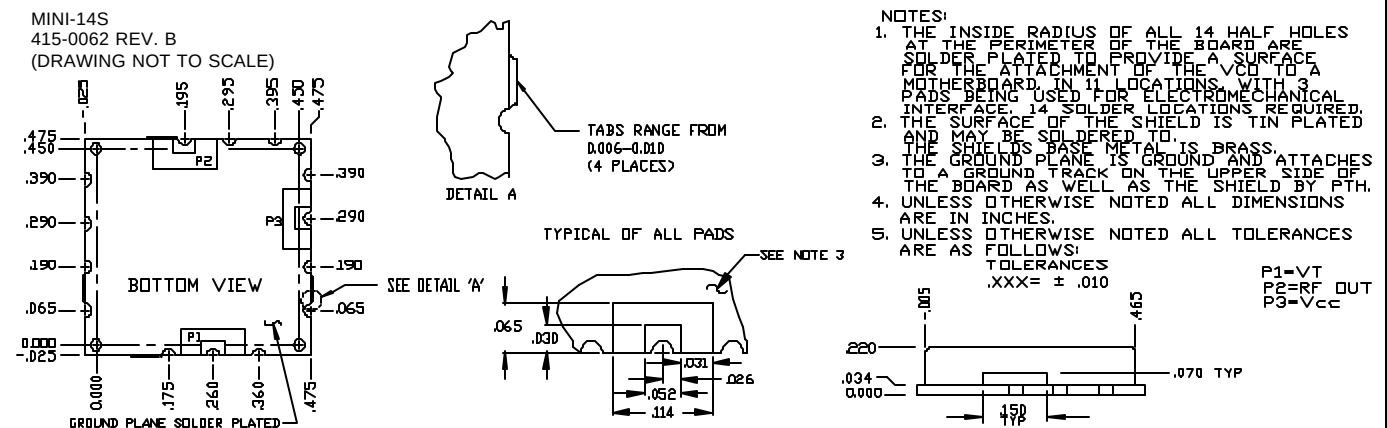
PHYSICAL DIMENSIONS
