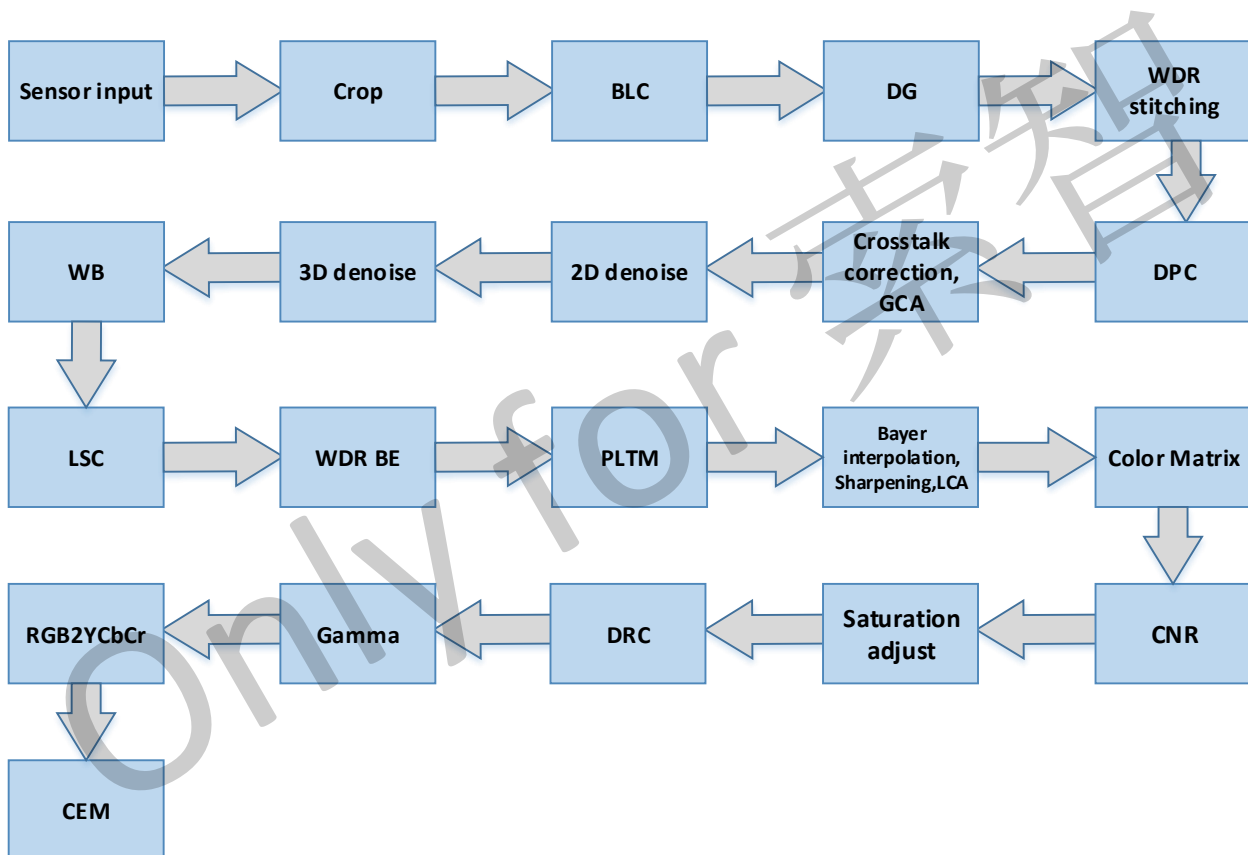
Figure 10- 1. ISP Block Diagram
