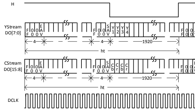
Figure 7- 12. BT.1120 60/50i Horizontal Timing Diagram
