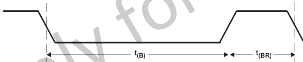
Figure 11- 36. Break Timing
