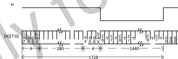
Figure 7- 16. 625line Horizontal Timing Diagram
