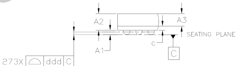
Figure 2- 4. Enlarged View of Detail "A"
