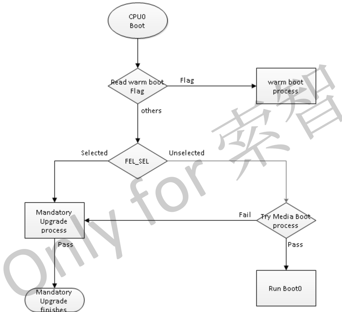
Figure 3- 6. Boot Process
