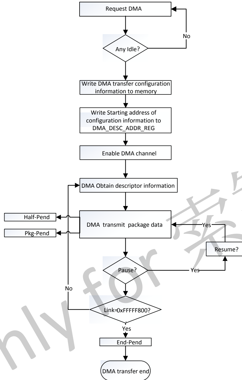
Figure 3- 24. DMA Transfer Process
