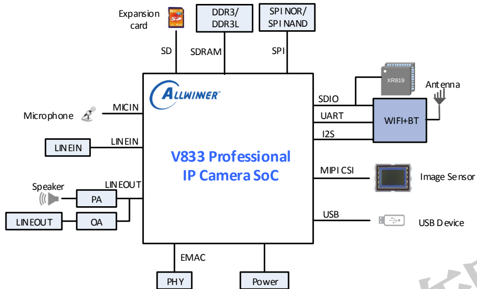
Figure 1- 1. V833 HD IP Camera Solution
