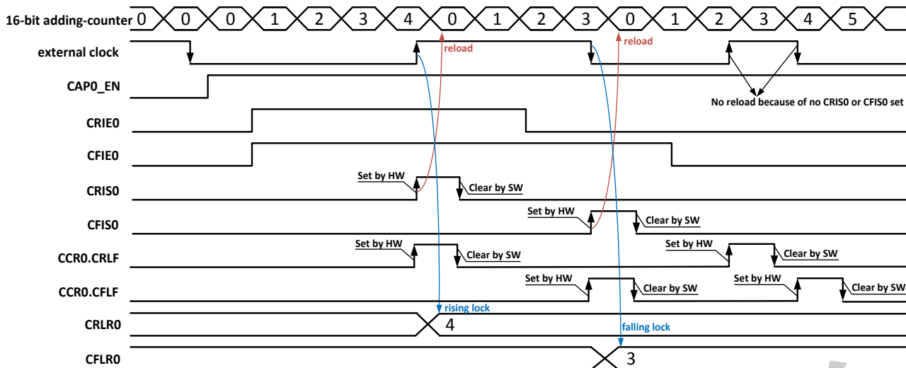
Figure 11- 62. PWM0 Channel Capture Timing
