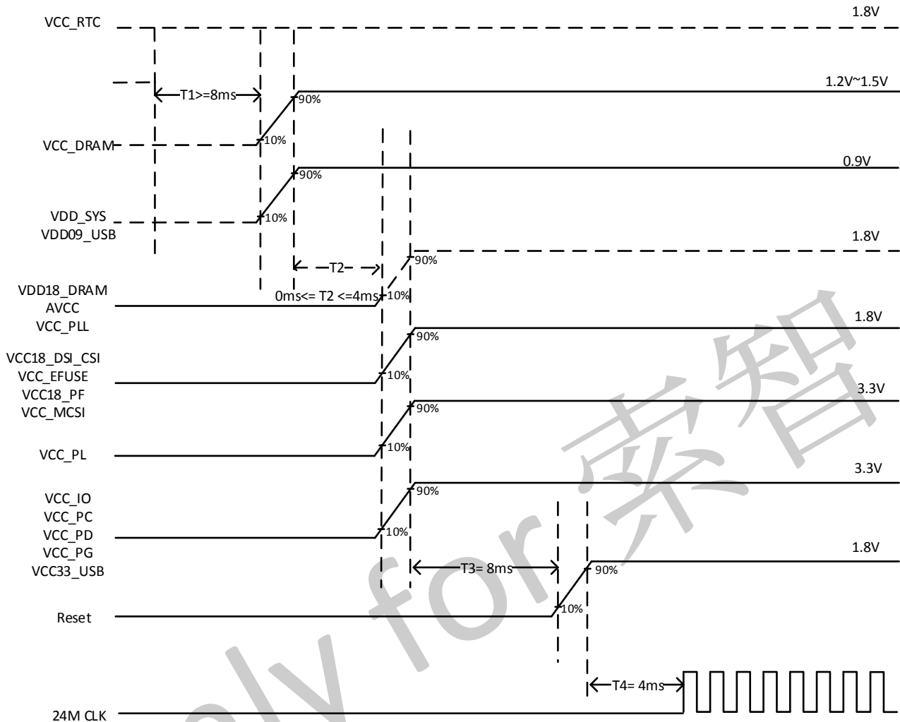
Figure 2- 11. V833 Power-on Sequence
