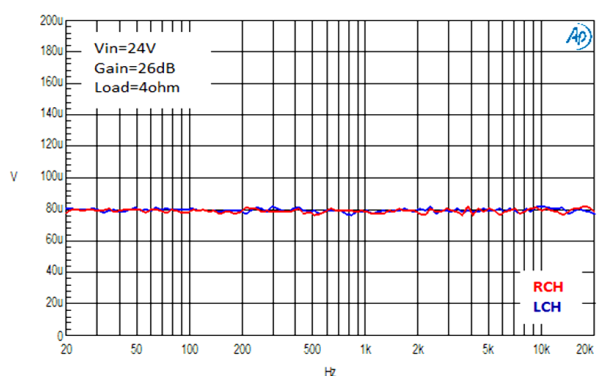
Figure 10. Noise, 24V, 4Ω load
