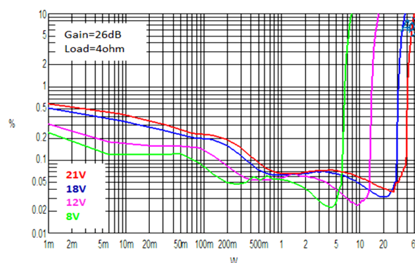
Figure 7. THD+N vs. Output Power, 4Ω load (BTL)
