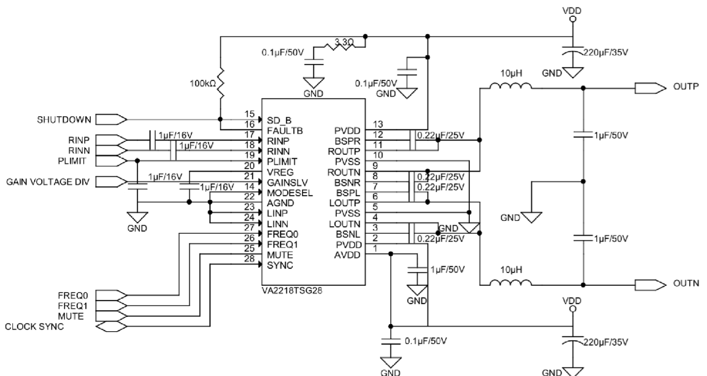
Figure 17. VA2218 TSSOP28 Mono Reference Application
