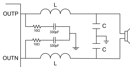
Figure 4. Output Snubber Circuits
