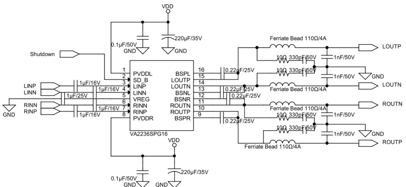
Figure 6. VA2236 Stereo Reference Application with Ferrite Bead
