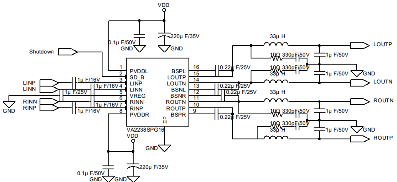
Figure 5. VA2238A Stereo Reference Application with LC Filter
