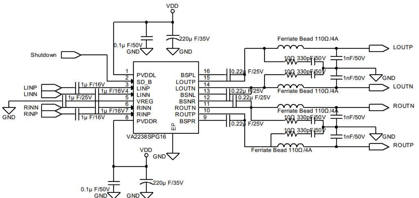
Figure 6. VA2238A Stereo Reference Application with Ferrite Bead
