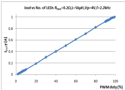
PWM duty vs. IOUT R_{SNS}=0.2\Omega, L=56\mu H
