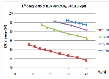
Vin vs. Efficiency R_{SNS}=0.1\Omega, L=56\mu H
