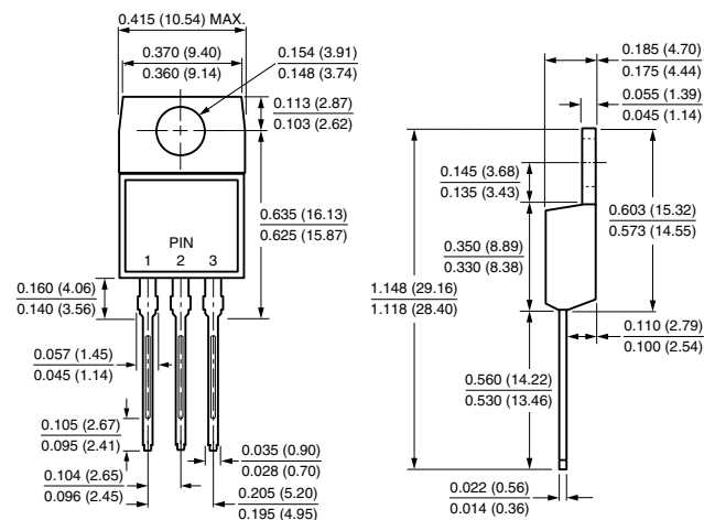
TO-220AB
