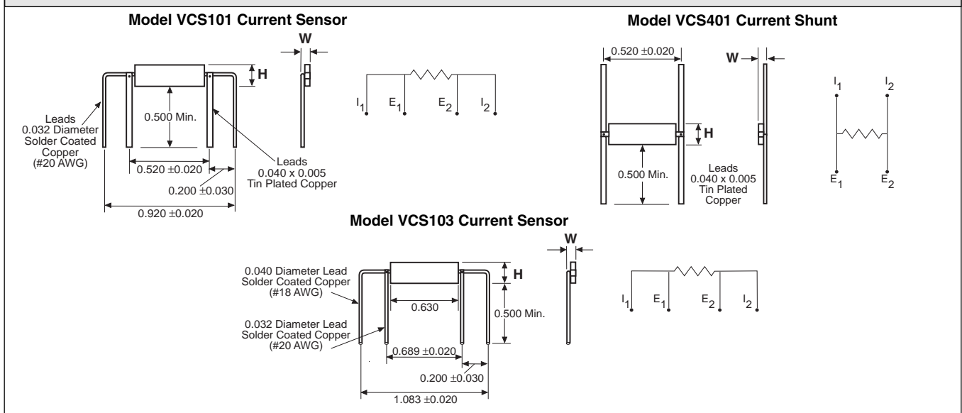
FIGURE 1 - DIMENSIONS AND SCHEMATIC
