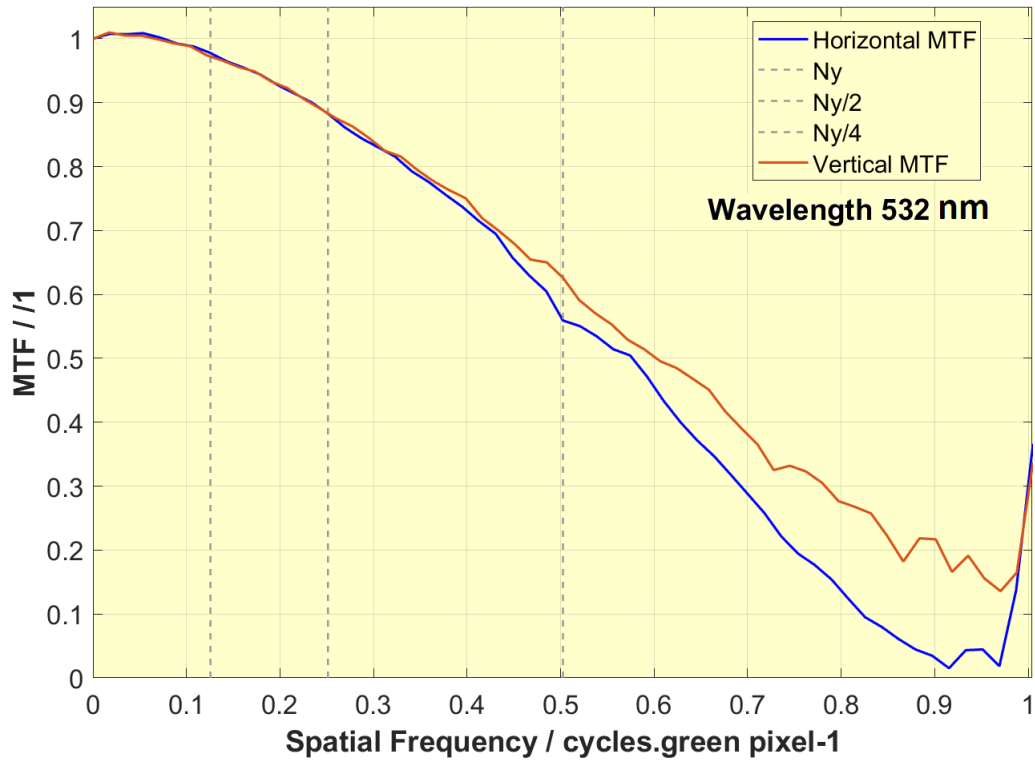
Figure 14. On-axis vertical and horizontal pixel MTF @ 532 nm
