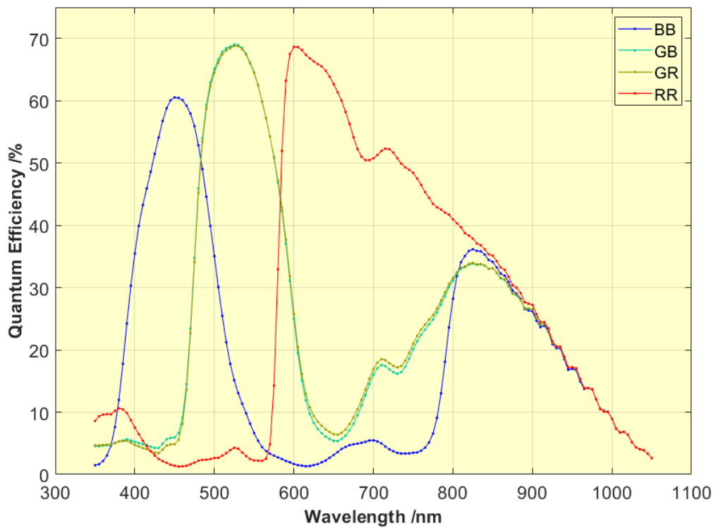
Figure 13. VD66GY RGB QE
