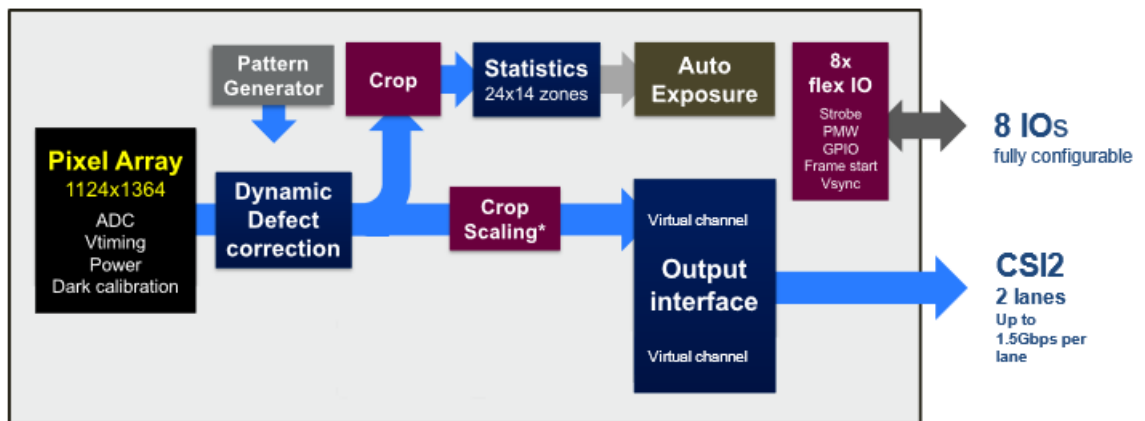
Figure 2. Image signal processor schematic
