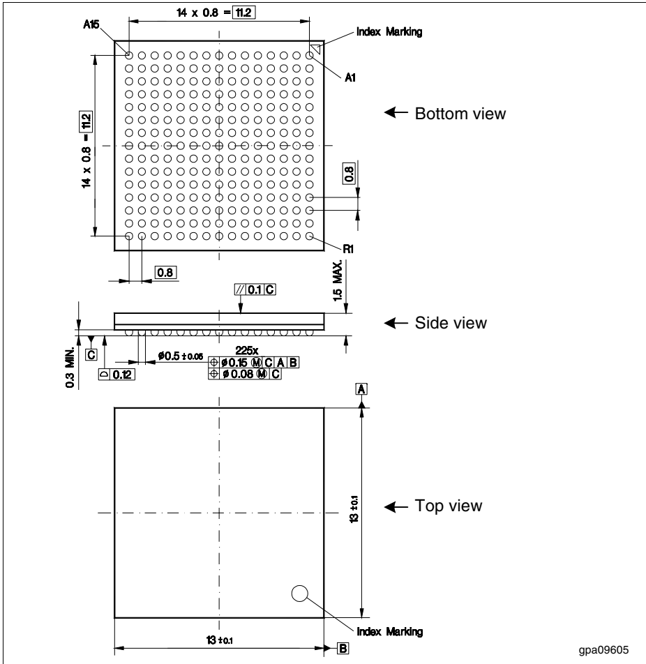
Figure 56 PG-LFBGA-225-1 Outline
