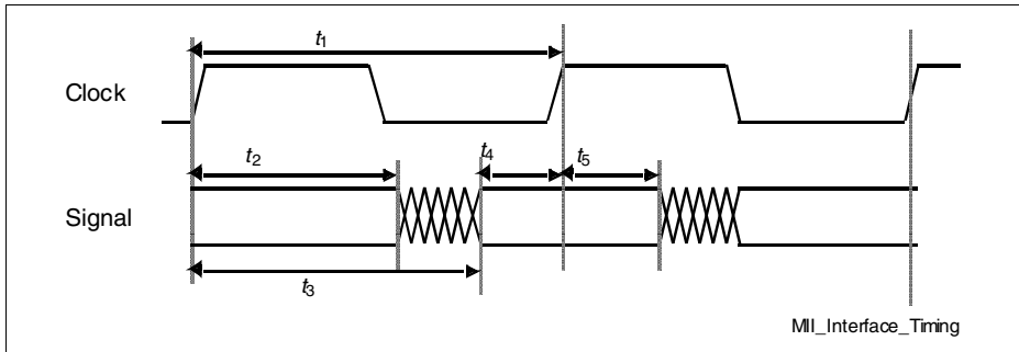
Figure 47 MII Interface Timing Diagram
