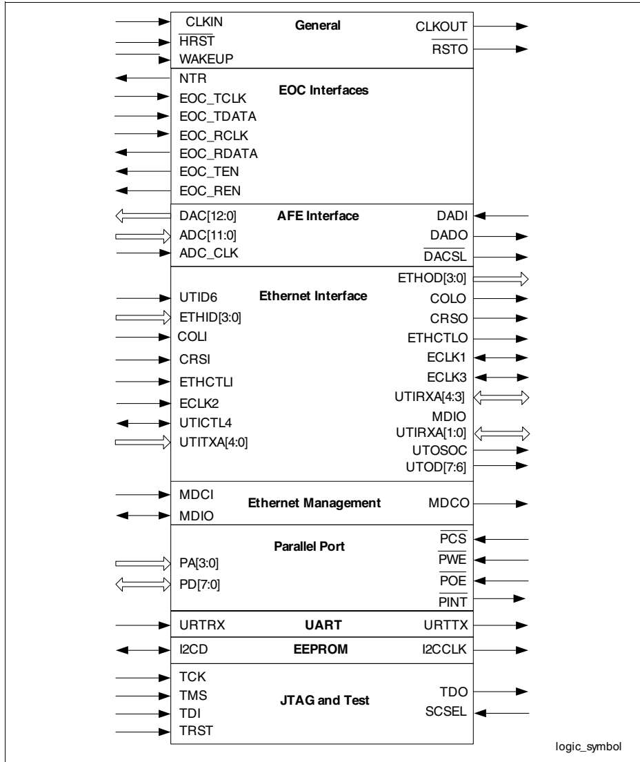
Figure 2 Logic Symbol
