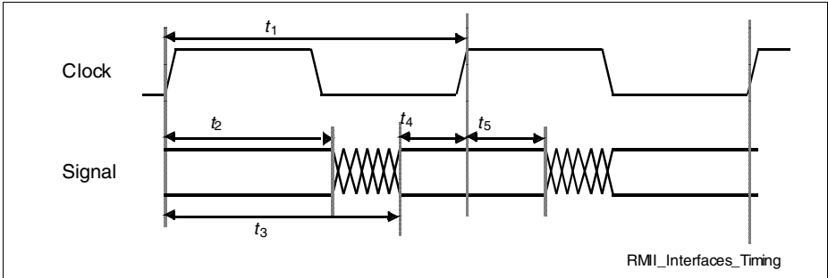
Figure 48 RMI Interfaces Timing Diagram
