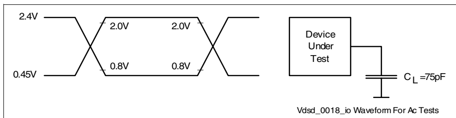
Figure 42 Input Output Waveforms for AC Tests
