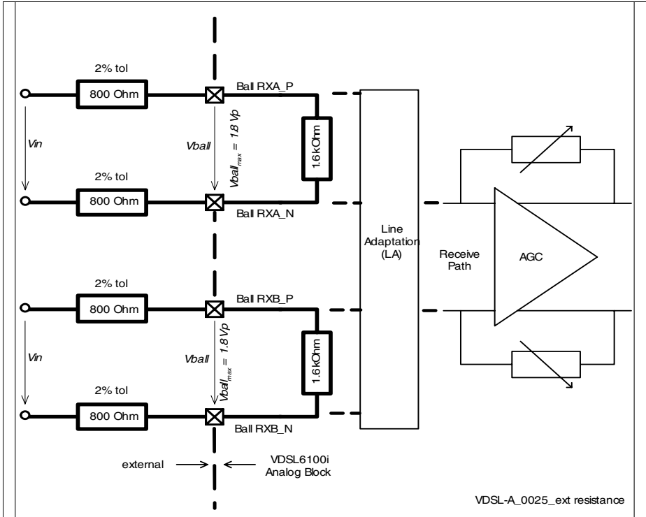
Figure 55 Input Resistance for Reception Input
