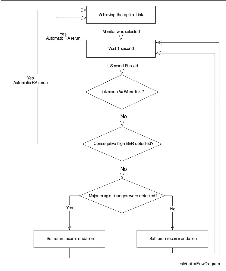
Figure 19 RA Monitor Flow Diagram
