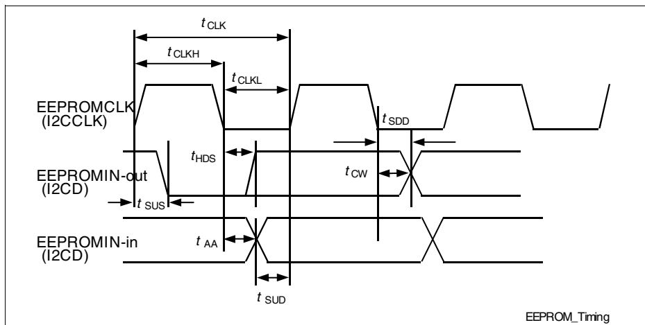
Figure 53 EEPROM Timing
