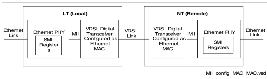
Figure 20 MAC-MAC Scenario
