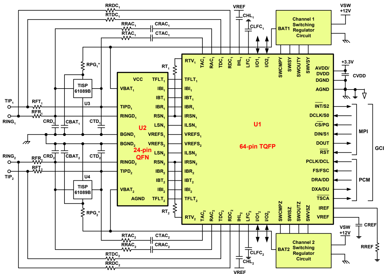
Figure 44. VE8820 Chipset Application Circuit
