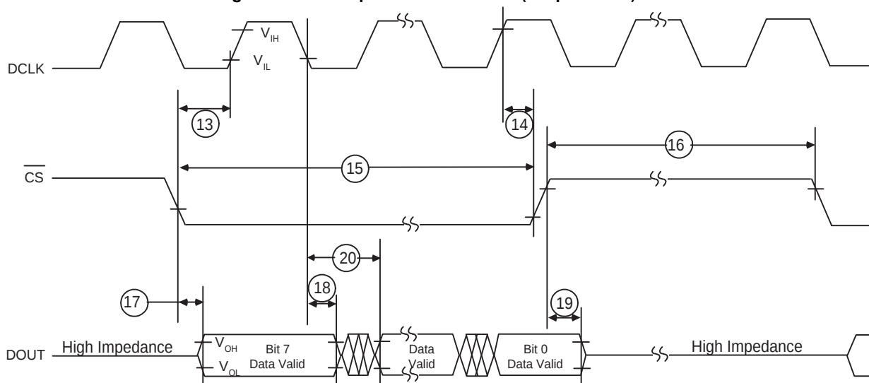
Figure 36. Microprocessor Interface (Output Mode)
