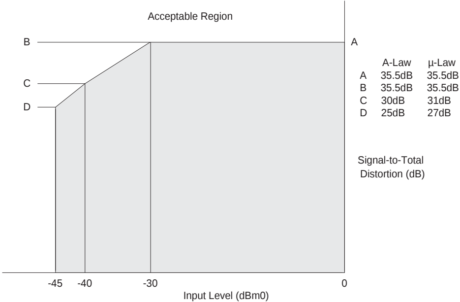
Figure 30. Total Distortion with Tone Input (Both Paths)
