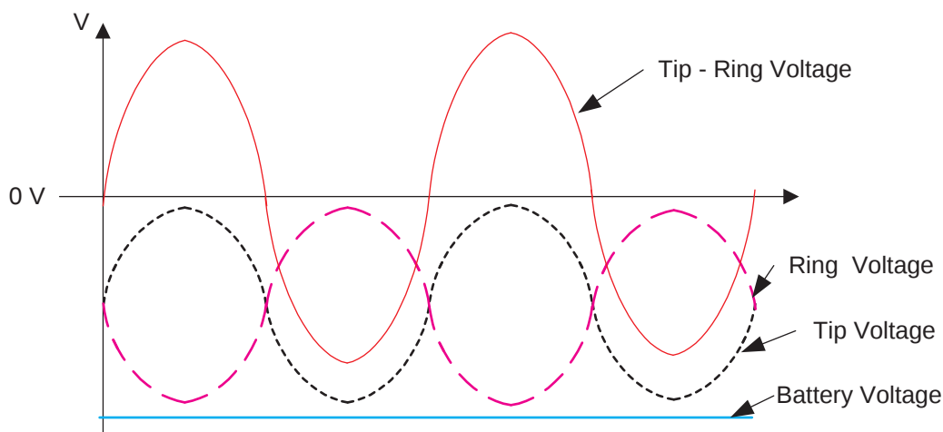
Figure 18. Balanced Ringing with Tracking Supply
