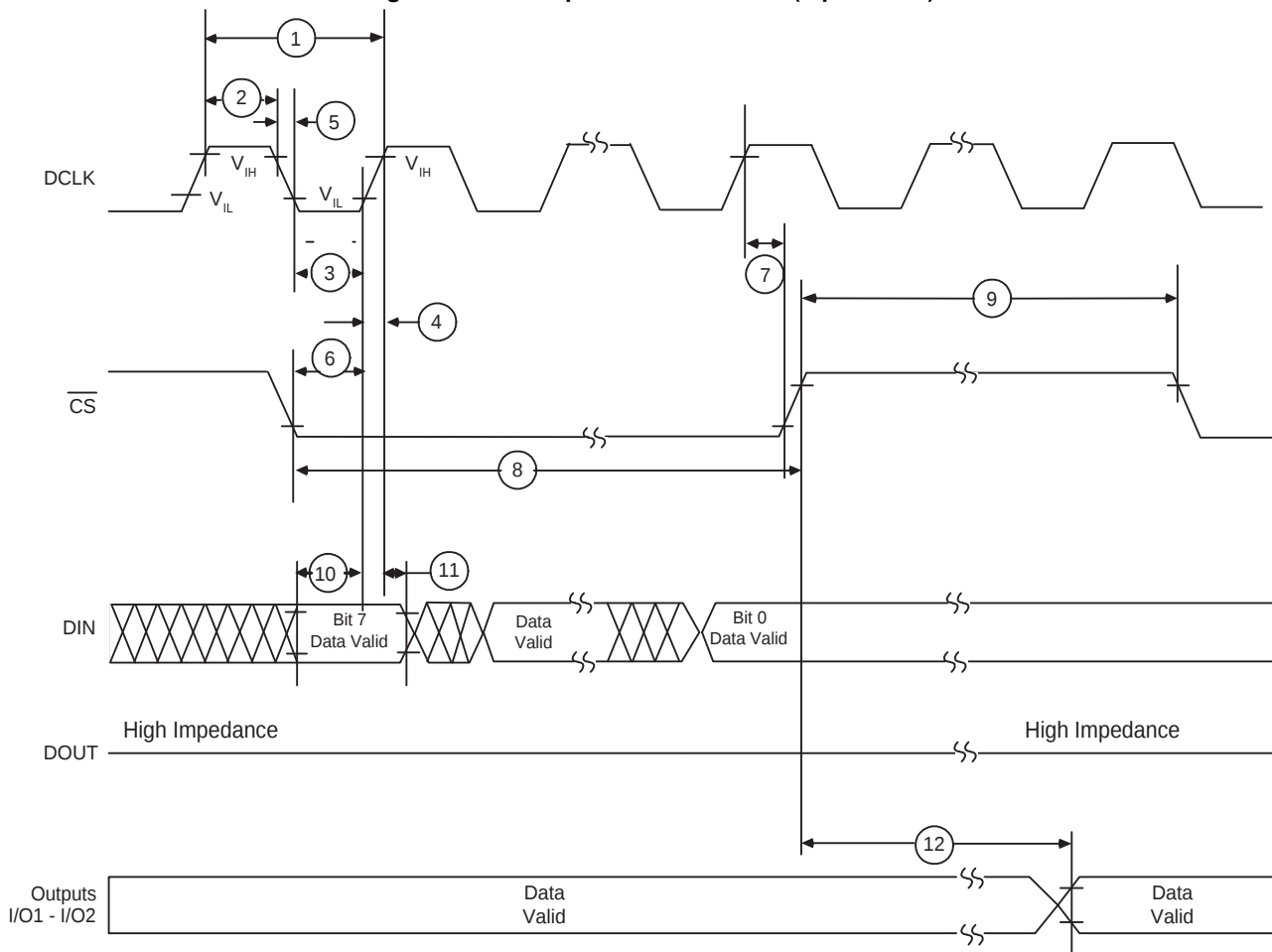
Figure 35. Microprocessor Interface (Input Mode)
