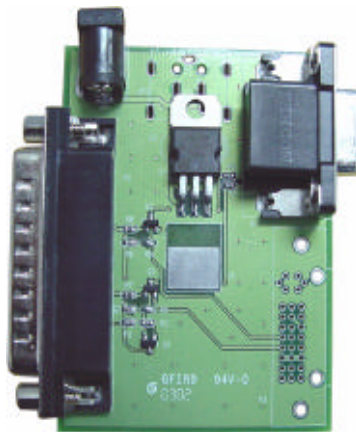
Fixture
