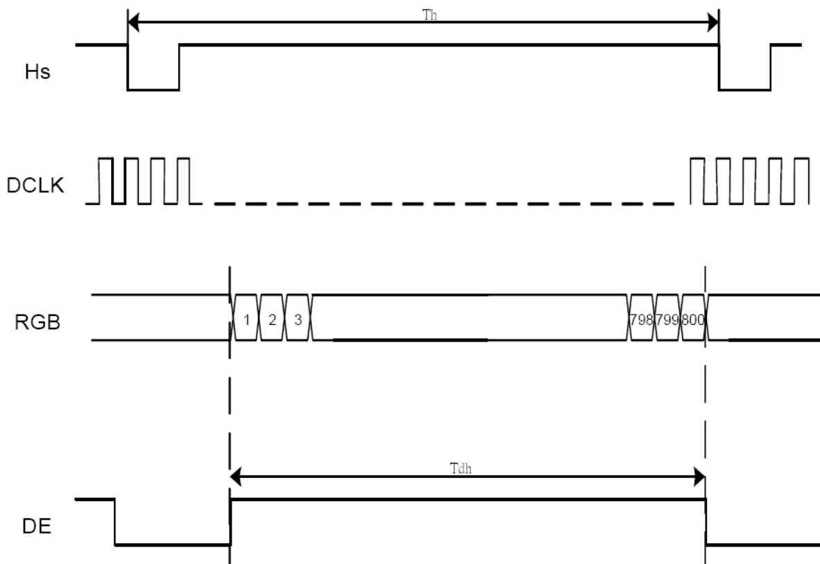
Fig.11.3-4 Horizontal timing 2
