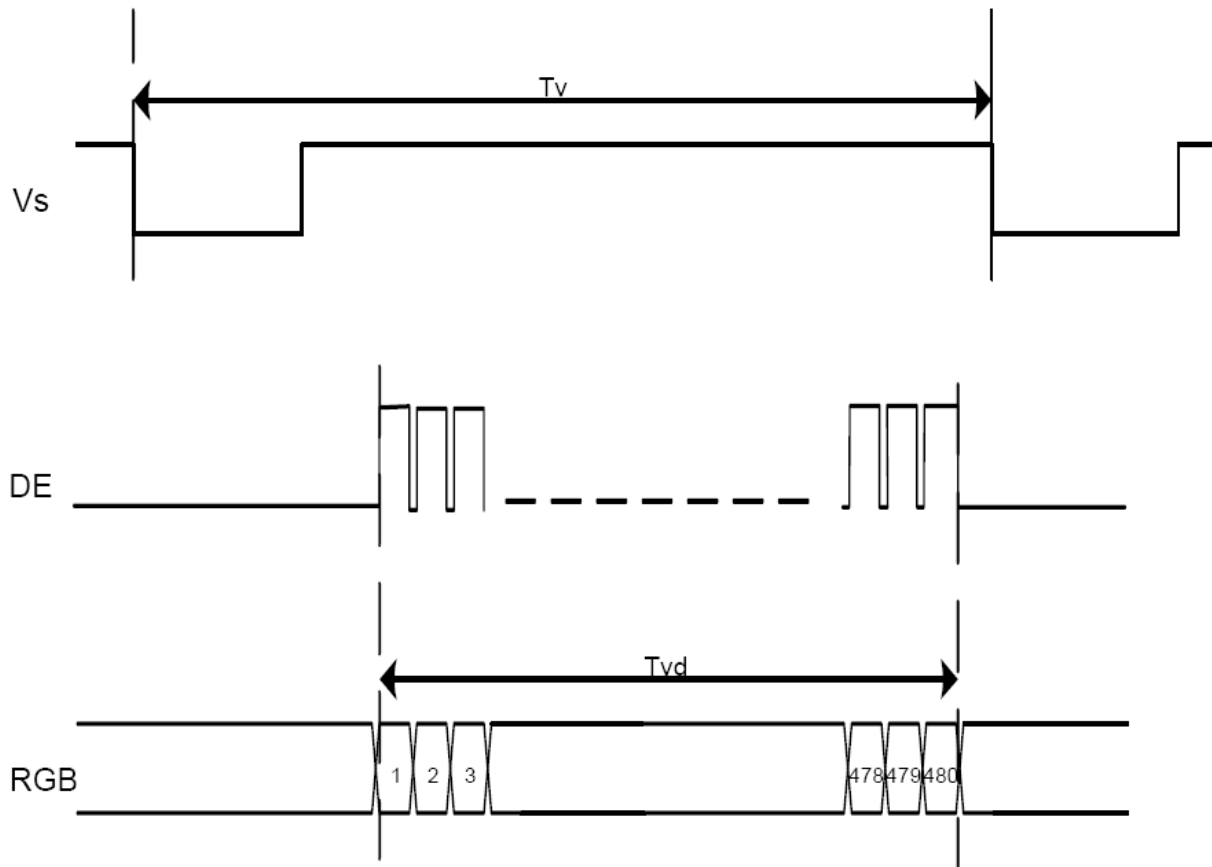
Fig.11.3-7 Vertical timing
