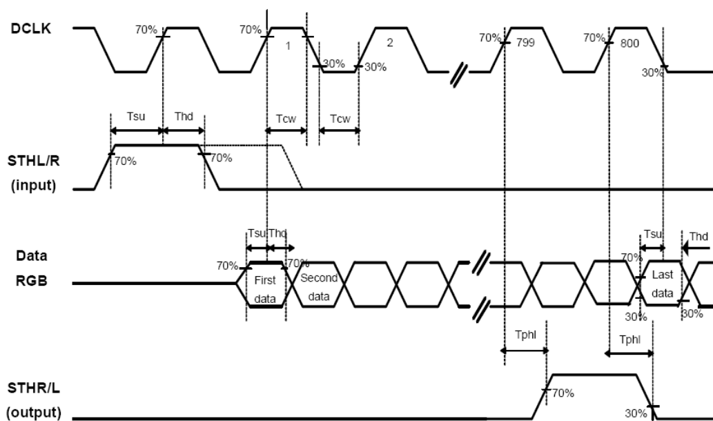
Fig.11.3-2 operation model 2
