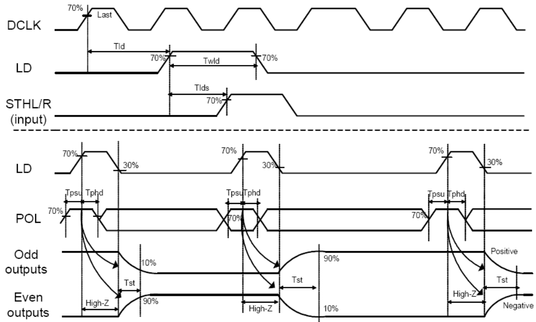
Timing Diagram 2
