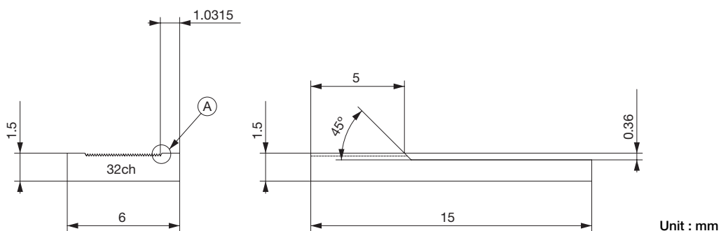
DETAIL A (20/1)
