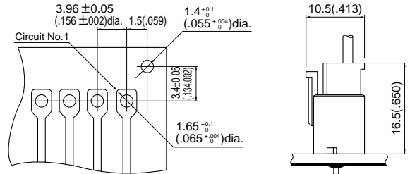
Shrouded header
