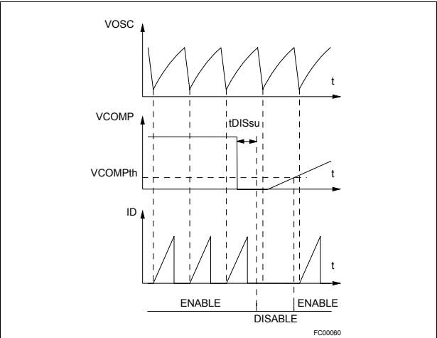
Figure 8. Shutdown action
