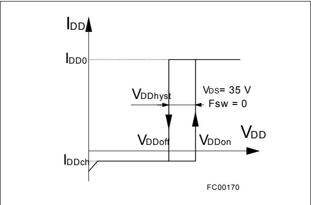
Figure 6. Undervoltage lockout
