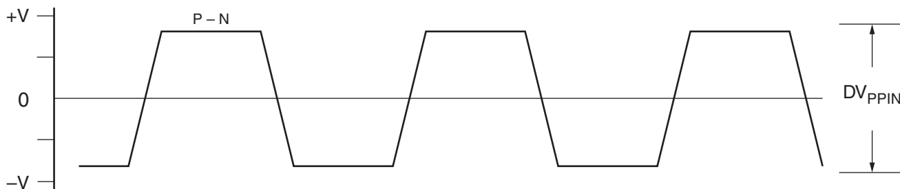
Figure 4: Differential Clock Input Voltage Swing Peak-to-Peak
