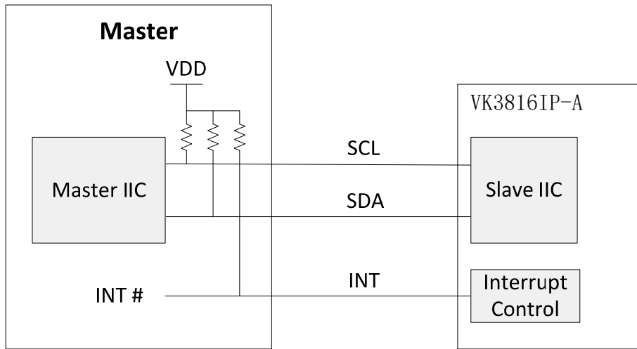
Figure6. IIC connect for master and VK3816IP-A
