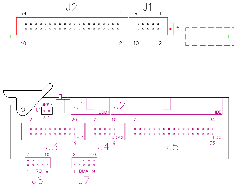
Figure 8. Connector Locations
