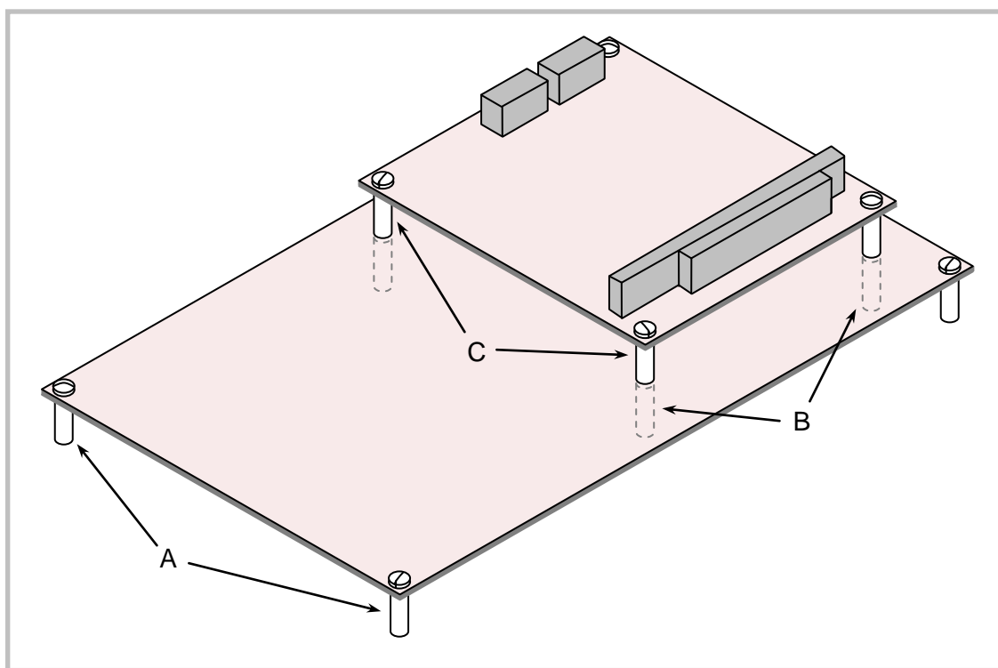
Figure 5. Standoff Locations
