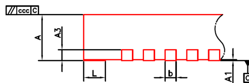
DETAIL : "B"
