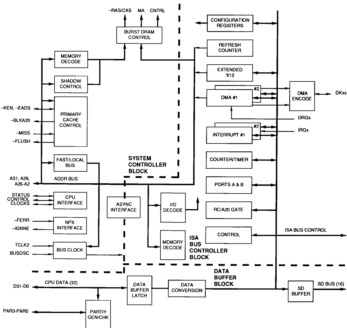
FIGURE 1. VL82C486 SUBSYSTEMS
