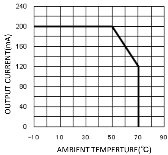
DERATING CHARACTERISTICS
