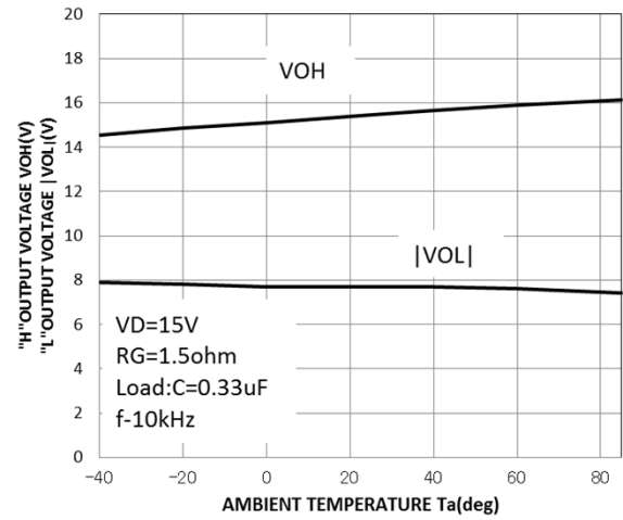
V_{OH} , |V OL | -T a CHARACTERISTICS (TYPICAL)
