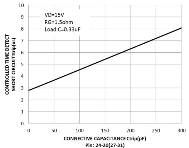
t trip -C trip CHARACTERISTICS (TYPICAL)
