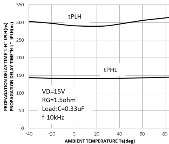
t PLH , t PHL -T a CHARACTERISTIC (TYPICAL)
