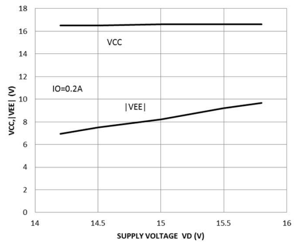
V CC , |V EE | -V D CHARACTERISTICS (TYPICAL)
