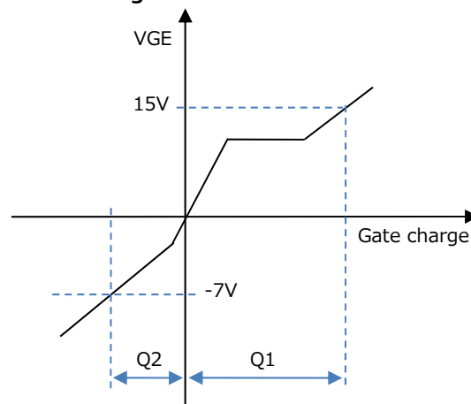
Gate charge characteristic of IGBT
