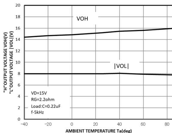
VOH, |VOL| -Ta CHARACTERISTICS (TYPICAL)
