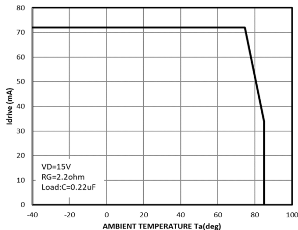
DERATING CHARACTERISTICS
