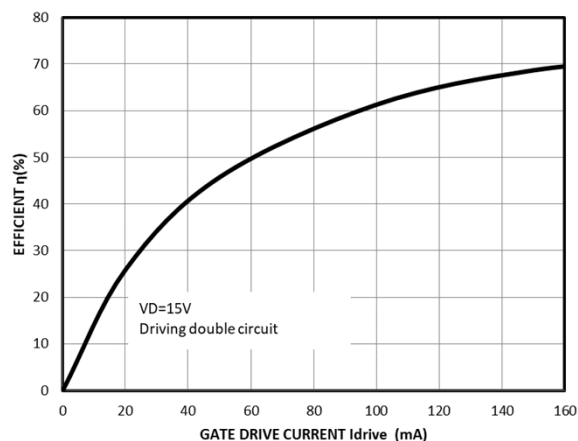
\eta-I_{drive} CHARACTERISTICS (TYPICAL)
