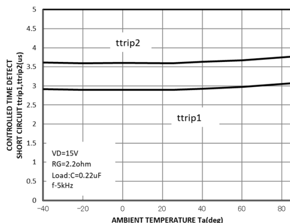
t_{trip}-T_a CHARACTERISTICS (TYPICAL)
