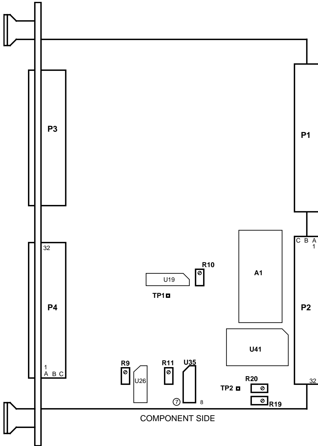
Figure 2-2 Locations of Test Points and Adjustments
