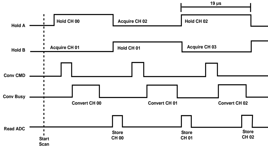
b. Scan Timing (Not to Scale)
