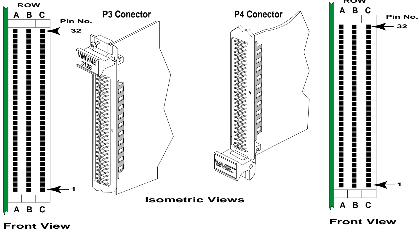
Figure 2-3 P3 and P4 Connector Pin Configuration
