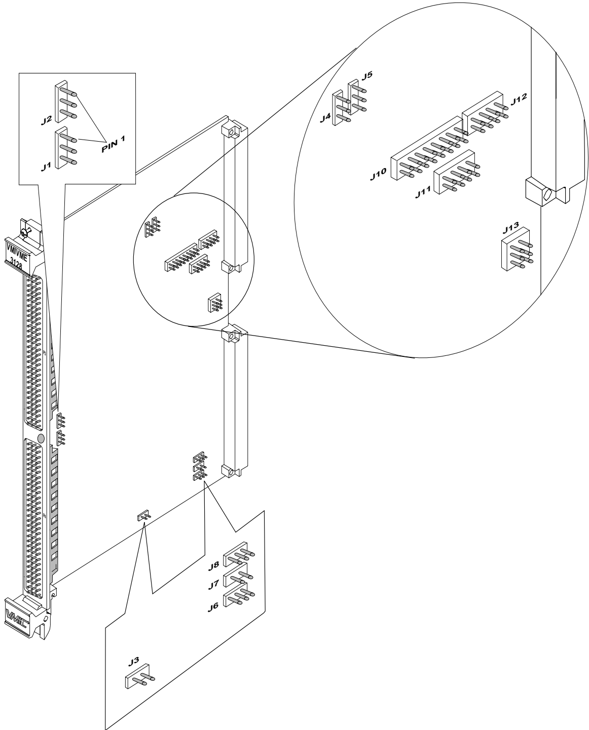
Figure 2-1 VMIVME-3128 Location of User-Configurable Jumpers
