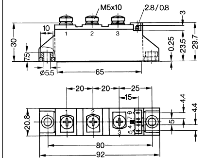
TO-240 AA Outline
