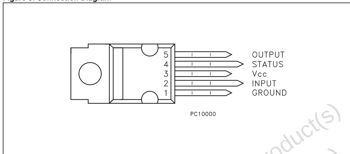
Figure 3. Connection Diagram
