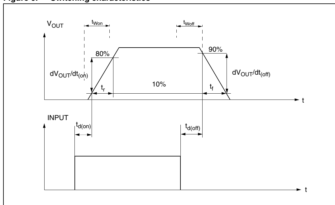
Figure 6. Switching characteristics
