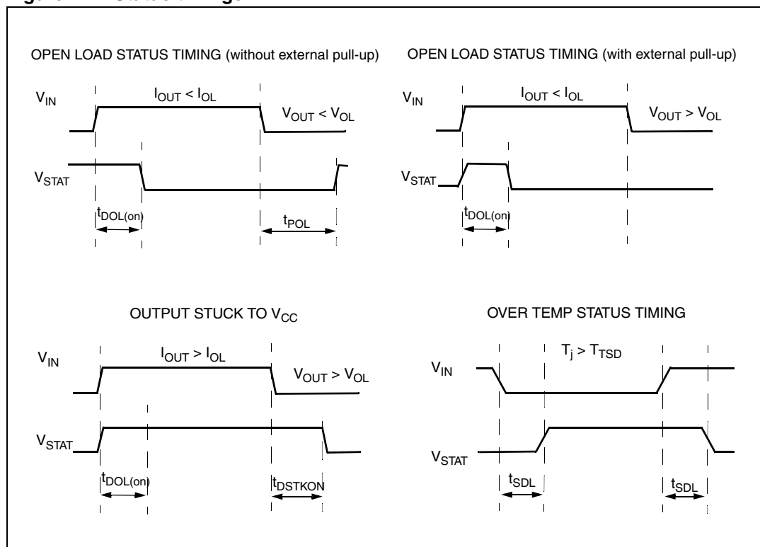
Figure 4. Status timings
