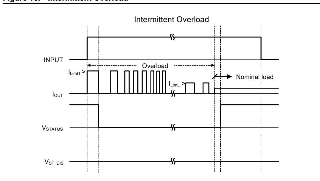
Figure 10. Intermittent Overload
