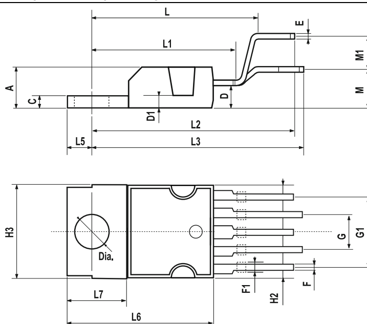
Figure 42. PENTAWATT (VERTICAL) Package Dimensions
