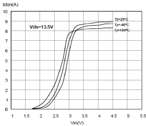
Figure 26. Transfer characteristics
