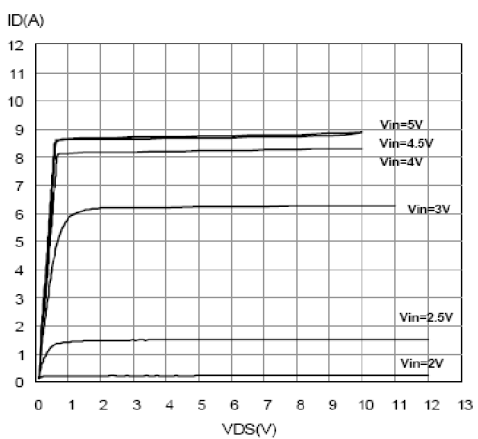
Figure 33. Output characteristics
