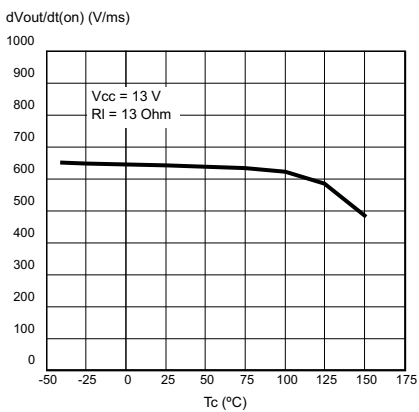
Figure 14. Turn-on voltage slope
