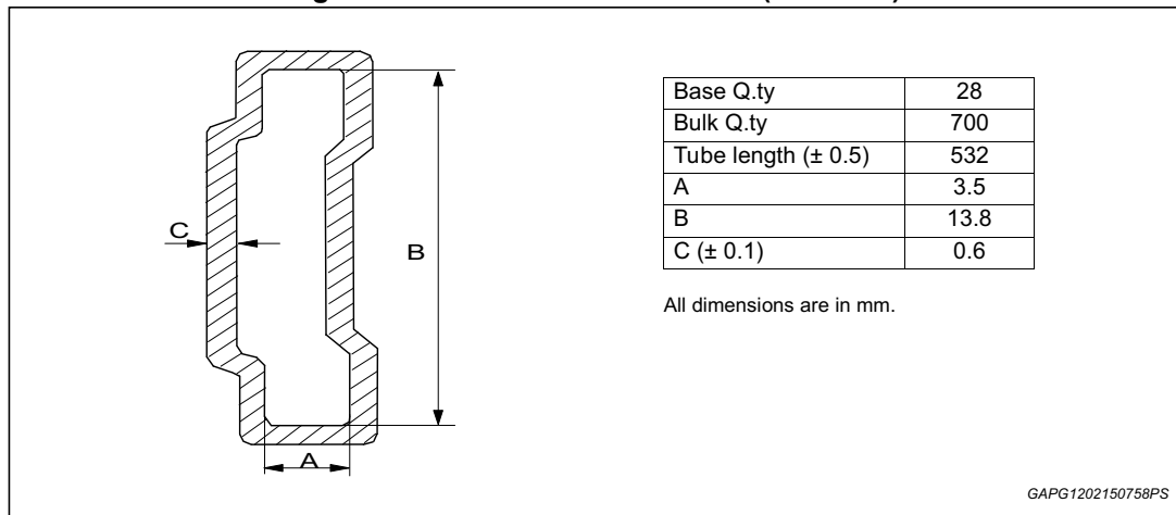
Figure 54. SO-28 tube dimensions (no suffix)
