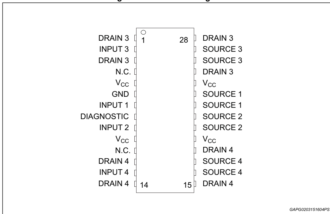
Figure 2. Connection diagram
