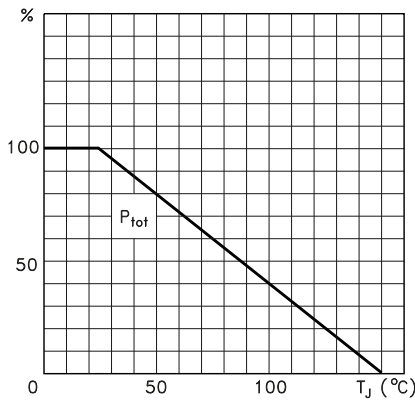
Figure 24. Derating curve
