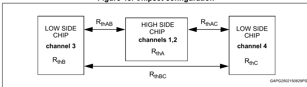
Figure 48. Chipset configuration
