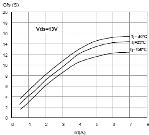
Figure 25. Transconductance
