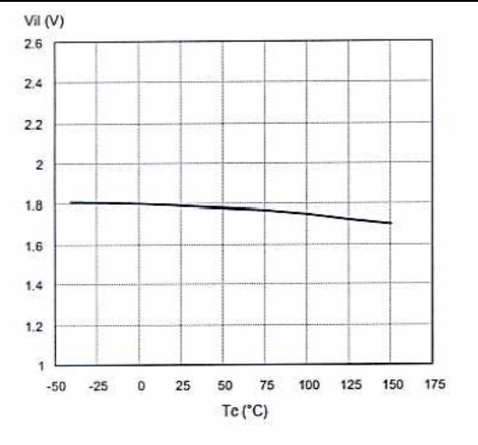
Figure 15. Turn-on voltage slope
