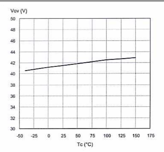
Figure 17. Overvoltage shutdown
